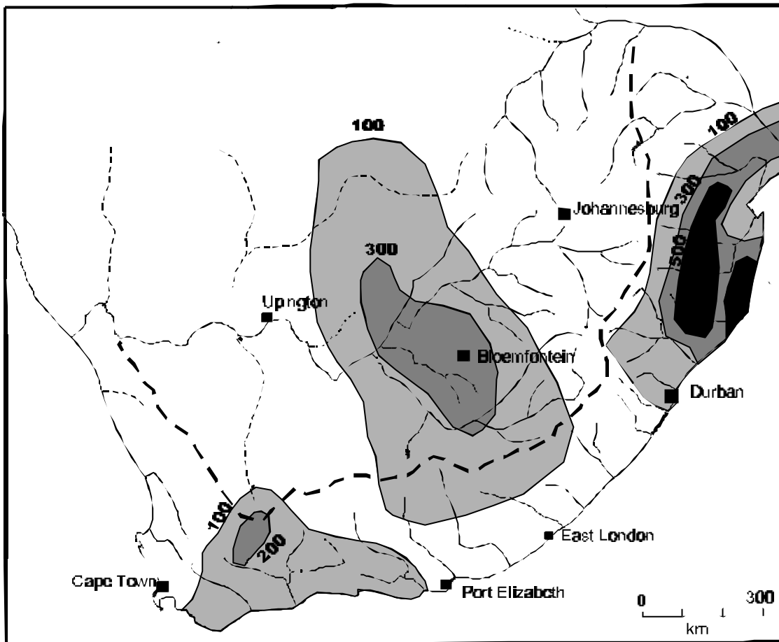
Figure 5 Location and properties of three typical widespread rainfall events
