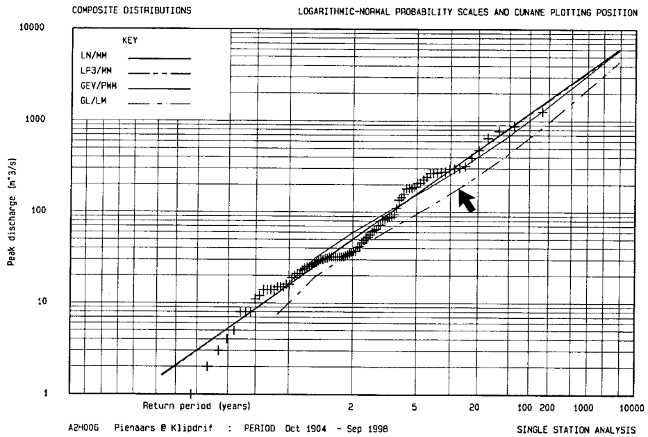
Figure 2. Combined distributions on logarithmic - normal distribution scales.
