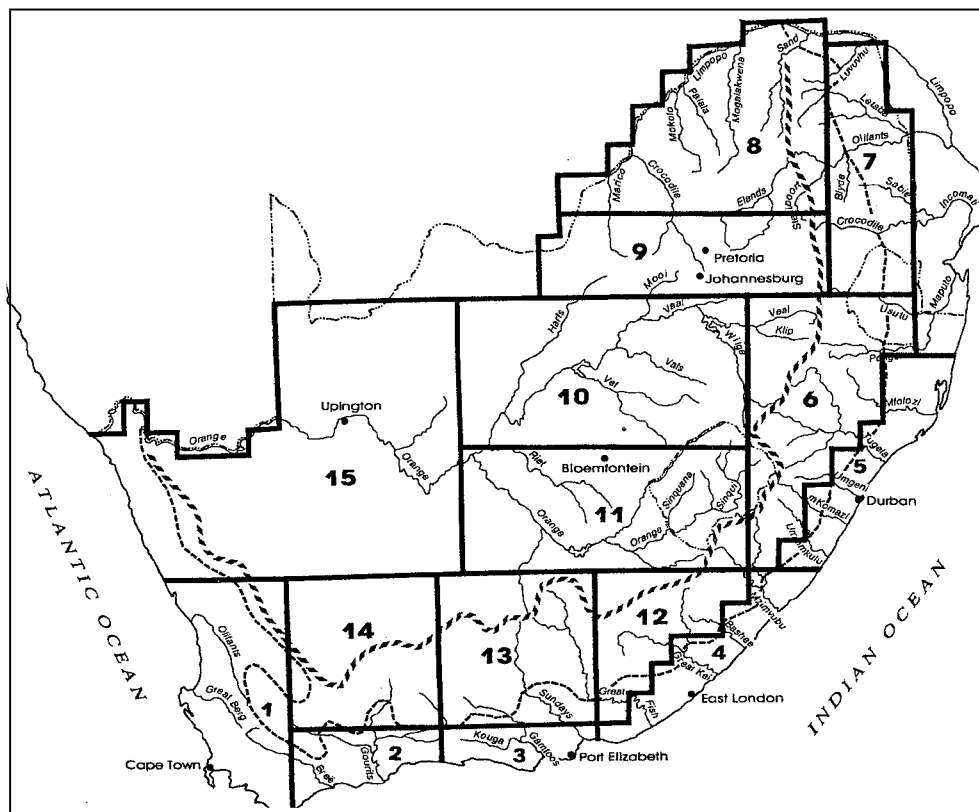
Figure 6. Regions used for widespread, severe rainfall classification.
