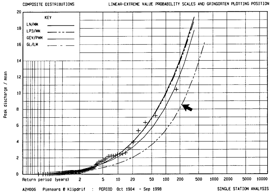
Figure 1. Combined distributions on linear - extreme value distribution scales.
