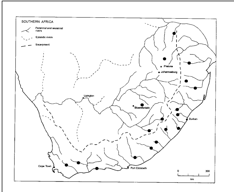
Figure 3. Location of the 18 stations used in the regional analysis.
